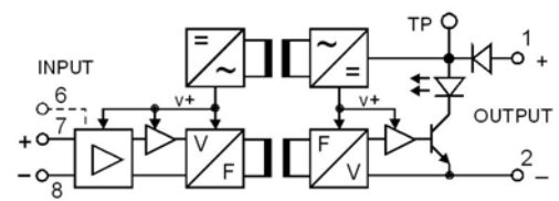
Block Diagram
