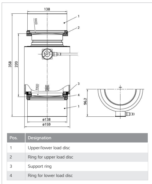
Load cell PR 6201/520 t (maximum capacity 520 t)
