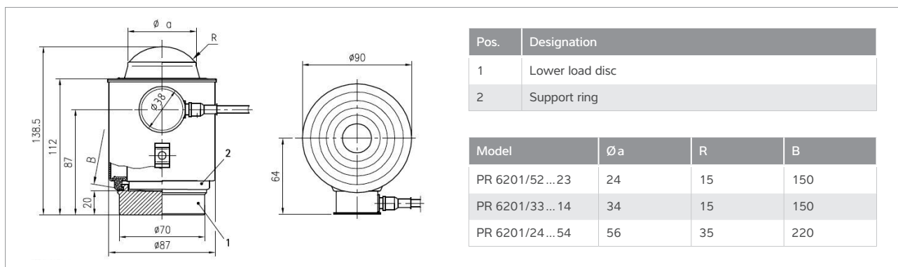
Load cells PR 6201/52...54 (maximum capacities 500 kg...50 t)
