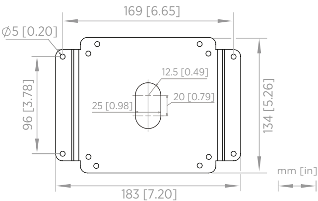
Indigo300 adapter plate (DRW257715SP) mounting dimensions
